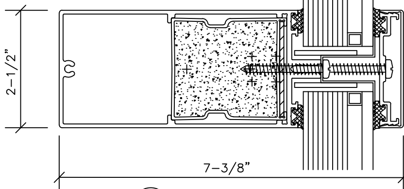
4 HOR. SECTION EXT. INSTALL
