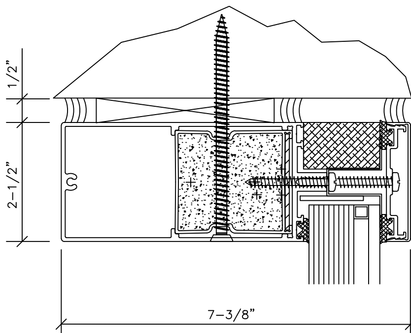
2 HEAD SECTION EXT. INSTALL
