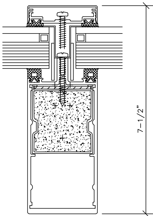
3 VERT. SECTION EXT. INSTALL
